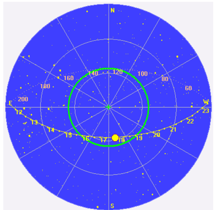
Sky map with riometer array HPBW in green.
