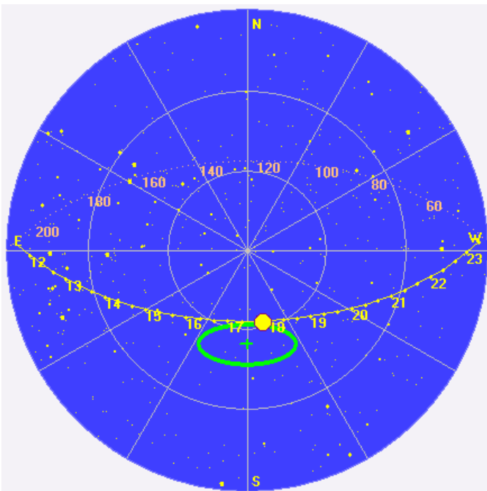
Sky map with TFD array HPBW in green.
